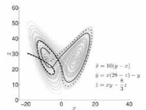
The Lorenz attractor found in models of a chaotic weather system has a characteristic butterfly shape. MacTighean CC BY
